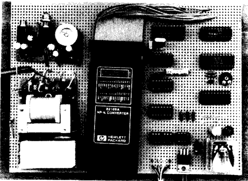
Photo of completed answering machine circuit. Hybrid transformer is shown in the lower left-hand corner.
