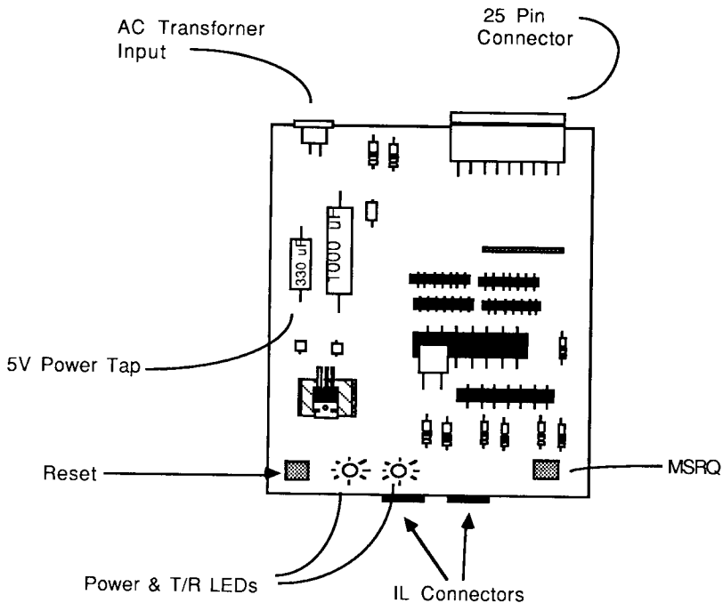
Figure 1-11 Power Tap inside the GPIO
