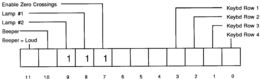
Figure 10-10 The OUT Register.
