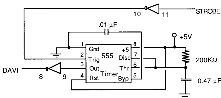
Figure 8-3 Pulse Expander
