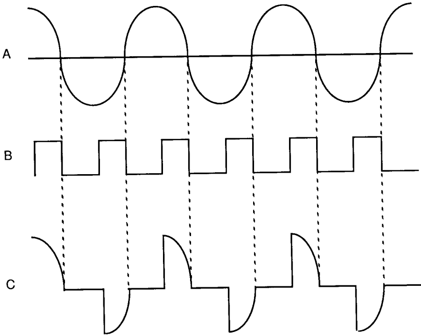
Figure 10-6 Clean Output.
